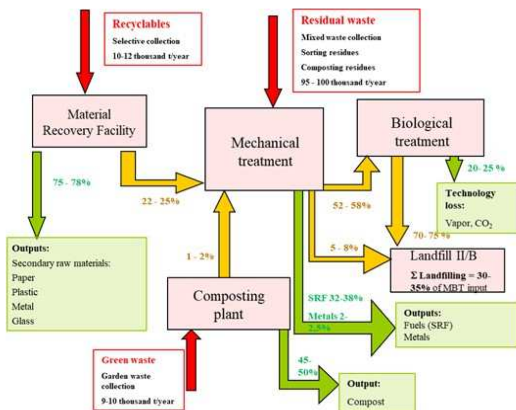
Figure 37: Internal waste streams of the Pécs-Kökény site
