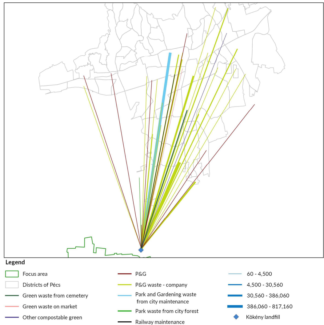
Figure 48: The material flow collected as P&G waste in Pécs agglomeration transporting to the Kökény composting facility (2017). It represents 1,547,600 kg P&G waste out of the 8,909,240 kg.
