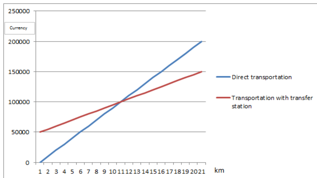
Figure 36. Drafted correspondence when to use direct transportation and transportation with transfer station in MSW transportation towards landfill/treatment.
